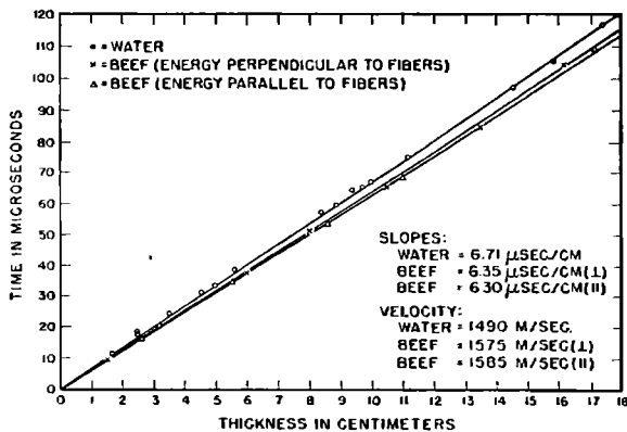
FIG. 2. Transmission time vs. thickness for distilled water and for beef. The velocity values calculated from the slopes of the lines are given in the lower right corner.
