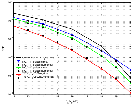
Fig. 3. The BER of TRPC and non-coherent systems in CM1 channels, with N_f = 4 .
